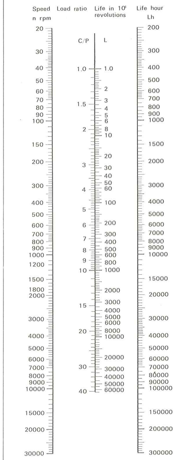
Fig. 2.1 NOMOGRAPH (n-C/P-L h )
