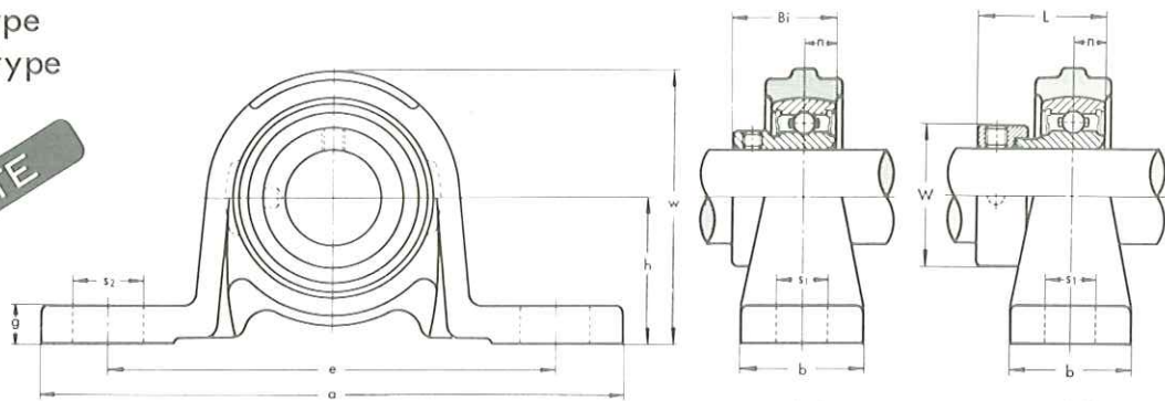
BPW 200 type
